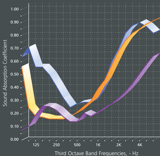
SOUND ABSORPTION COEFFICIENTS OF 1/2"(13mm) ALUSION PANELS ON "E-400 MOUNT" (OVER 16" SPACE)
